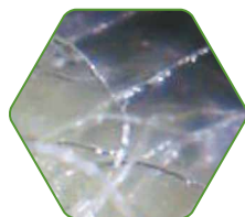
MÉLANGE CONCURRENT
